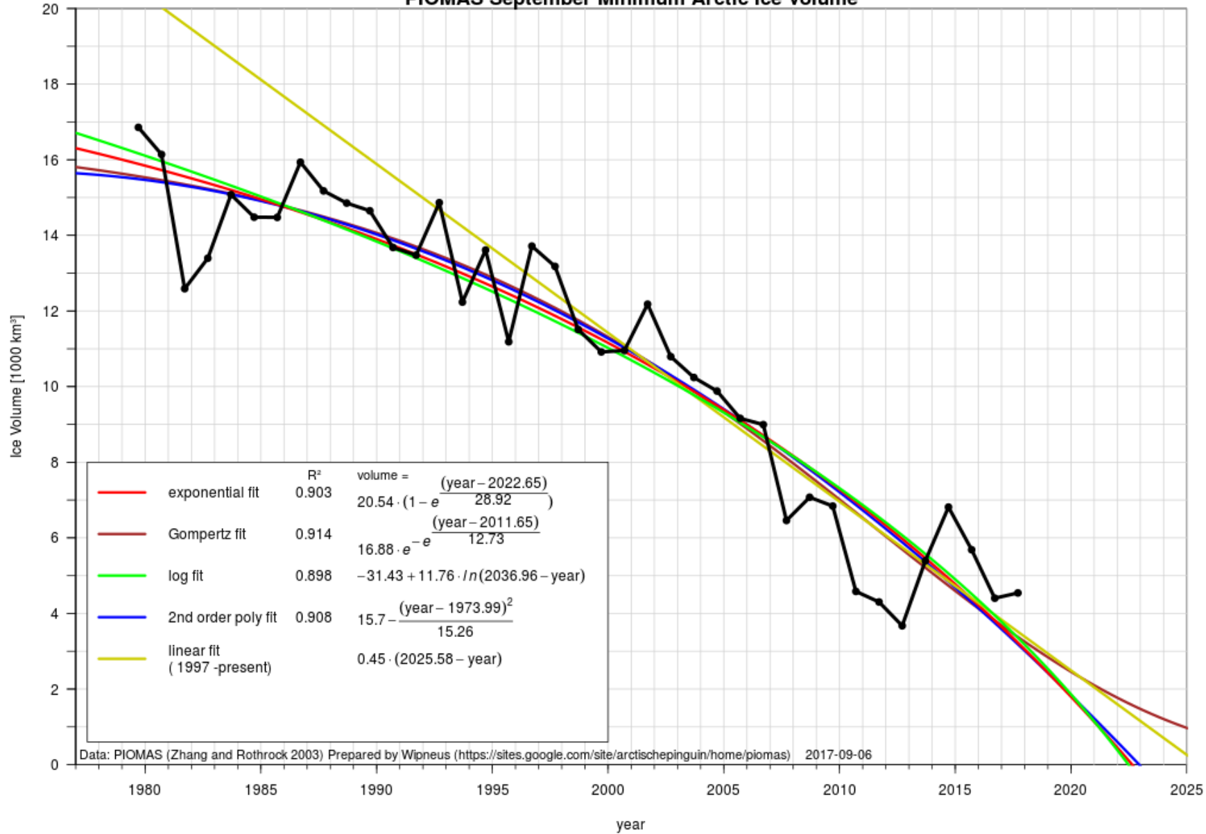
PIOMAS September Minimum Arctic Ice Volume
